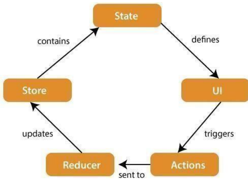
Fig 4.1 Redux Architecture
